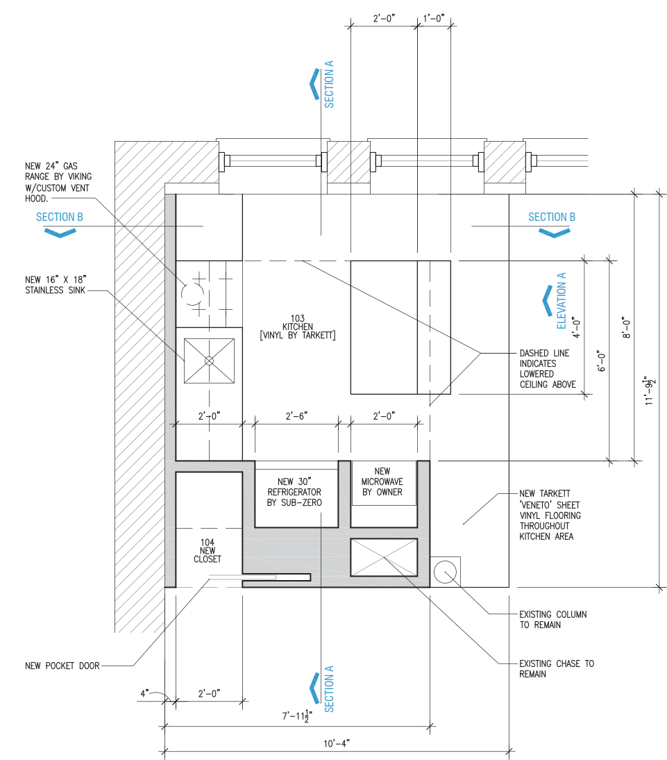
FLOOR PLAN
