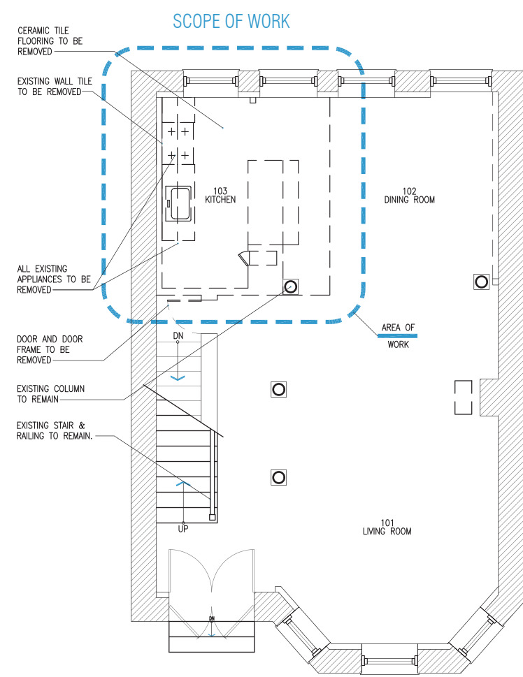
REFERENCE PLAN
